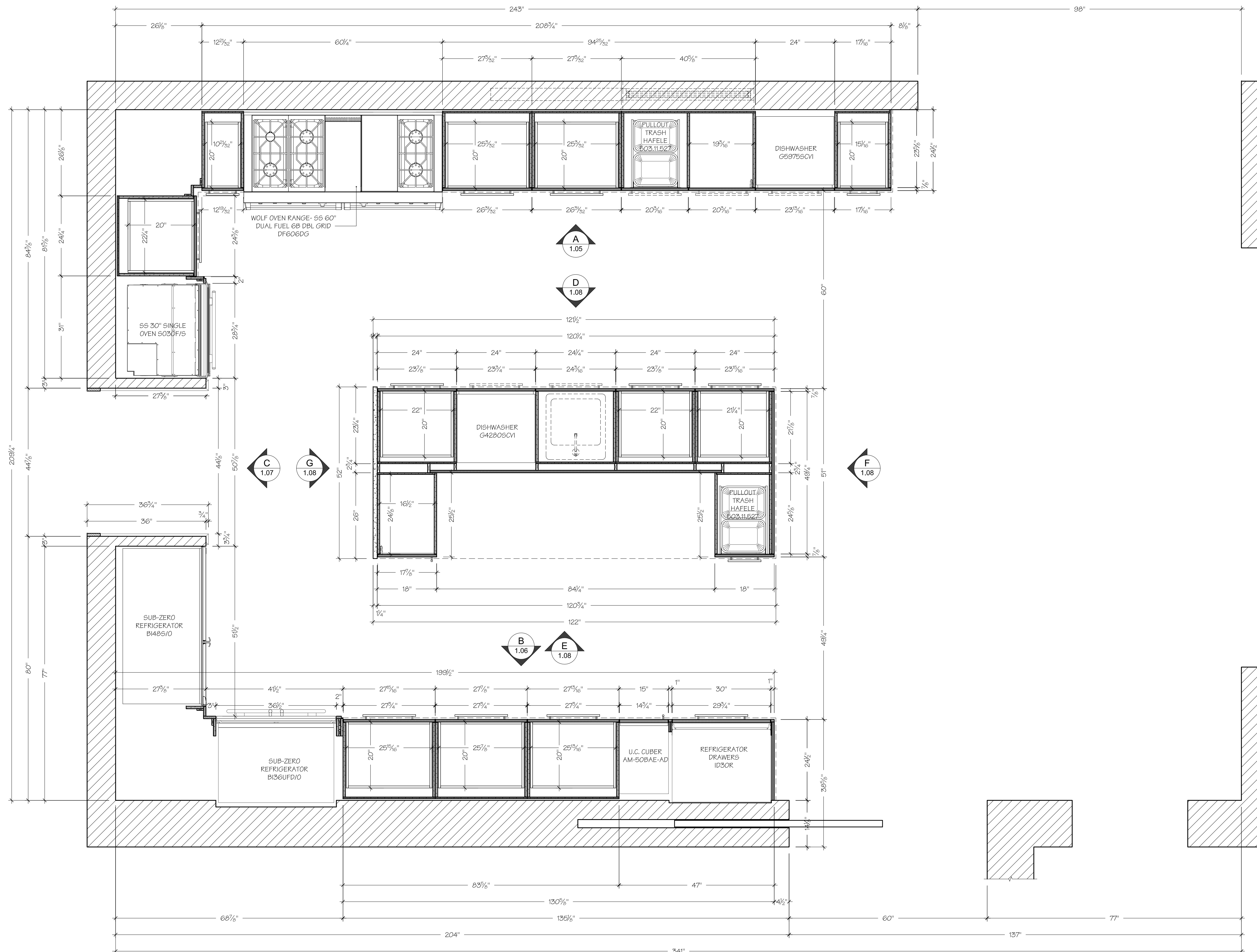
1 SECTION PLAN SCALE: 3/4" = 1'-0" KITCHEN
